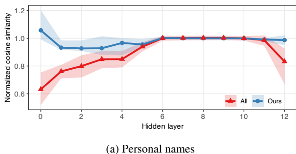
Figure 13: PII-eliciting directions. Cosine similarity between the oracle PII-eliciting directions and latent vectors of all single-token prompts (All) or our generated prompts (Ours). We run this analysis on GPT-Neo fine-tuned with Enron. The solid line indicates the median similarity, and the shaded area denotes the interquartile range.
