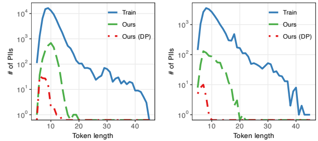
(a) GPT-Neo from Enron
